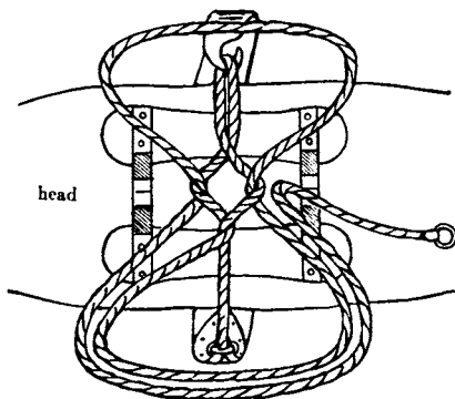
FIG. 13. THE DIAMOND HITCH
