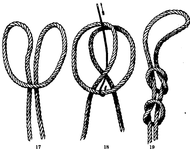
FIGS. 17, 18, 19. STEPS IN TYING THE FISHERMAN'S BEND
