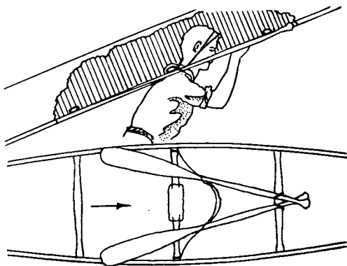
FIG. 9. CARRYING RIG FOR CANOE
