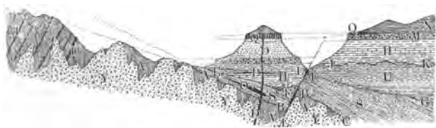
FIG. 32. DIAGRAM OF GEOLOGICAL STRUCTURES
