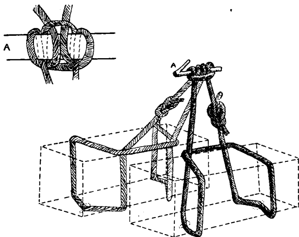
FIG. 16. METHOD OF SLINGING TWO CAMEL-BOXES
