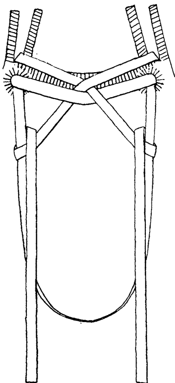
FIG. 4. SNOWSHOE TIE WITH FIXED TOE STRAP
